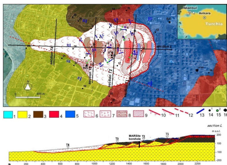
Figure 7. Example of reconstruction of the geological structure of the Büyükçekmece slope (Turkey) with identification of the materials and the different phases of reactivation of the ground movement. The top figure shows an image of the site with the plan outlines of the moving area. Several two-dimensional sections (black lines) have been defined in this image to reconstruct the geological structure of the slope. As an illustration, the bottom figure represents the longitudinal section constructed in the direction of movement to analyze the causes behind the reactivation of this ground movement. On this section, the different materials are represented by colours: brown clay deposits, red sands and gravels, blue limestone arenites and yellow silty clays. The red lines represent the sliding surfaces identified on this site and reflect the different phases of reactivation of the ground movement: throughout its history, instability, which began to develop at the foot of the slope, has spread towards the crest of the slope. [© Salvatore Martino, with permission; see reference 16]
