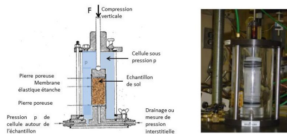
Figure 4. The triaxial test is used to characterize the rigidity and strength of a deep soil. On the left, the principle of the test (metrology not shown). On the right, picture of a triaxial cell. The cylindrical sample is subjected to a confinement stress p (simulating depth), then compressed (axial force F representing the action of a nearby structure), from small deformations to failure. [© Marc Boulon]
