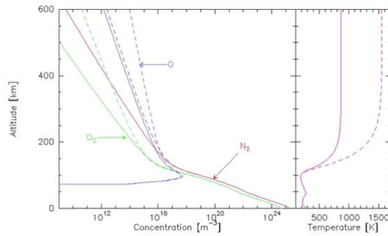
Figure 2. Upper atmosphere section at medium latitude ( 45^\circ N). On the left, concentration of the majority of neutral species up to 600 km above sea level. On the right, neutral temperatures. In full line, typical values for a calm Sun. In dotted lines, typical values for an active Sun.
