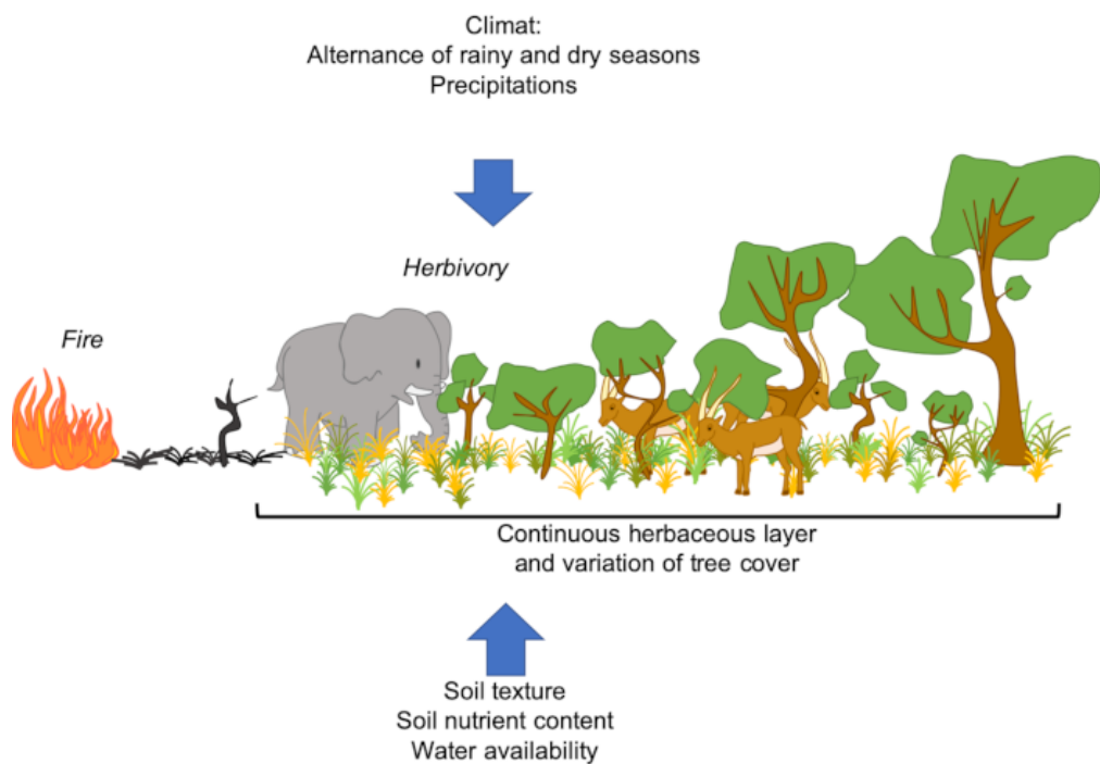
Figure 4. Diagram of savanna organization with a continuous herbaceous layer with mostly C4 grasses, many forbs (non-woody herbaceous plants other than grasses), and the presence of more or less or less tree and shrub species. The two main disturbances of these vegetation are recurrent fires and herbivory, although herbivory pressure is not the same all over the world. [Source: © S. Le Stradig & E. Buisson]
