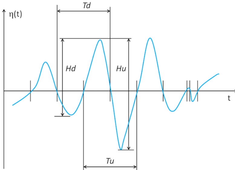
Figure 10. Wave height estimation [Source: Nielsen P, Coastal and estuarine Processes, Advanced Series on Ocean Engineering vol, 29, DOI:10.1142/9789812837134_0001 ]
