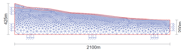
Figure 3. Mesh size for the study of a landslide at Petacciato (Italy) - by the numerical finite element method - with an average slope of 6^\circ . [Source: PhD thesis by Florent Prunier, Grenoble INP, 2008. Available online: https://tel.archives-ouvertes.fr/tel-00355769/document ]
