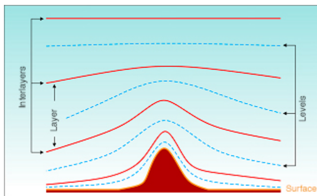
Figure 5. Diagram showing a common example of vertical discretization of the atmosphere. The levels where the average parameters calculated by the model are positioned are drawn in blue. These levels follow the terrain when they are near the surface and become horizontal at higher elevations. The parameters calculated on the levels of the model represent an average value in a layer, limited on this diagram by red lines (See ref.[3]) [Source: Malardel, 2009.]
