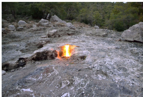
Figure 3. Flaming release of a mixture of methane, ethane, propane and dihydrogen from serpentine soil in southern Turkey. This site, named "la Chimère" proves the reality of organosynthesis reactions such as Fischer-Tropsch, since they take place nowadays in the Turkish subsoil [Source : photo Pierre Thomas]
