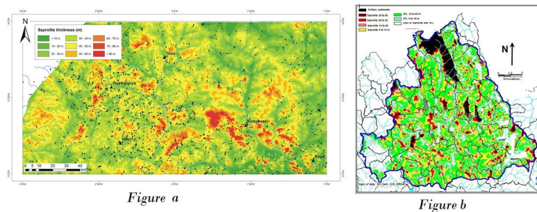
Figure 7. Examples of maps at different scales of the different constituent layers of basement aquifers. Figure a: Thickness of saprolite over a region of about 250 x 100 km in Burkina Faso[8]. Figure b: geological map of the entire alteration coverage over the Lozère basin of the Truyère (Lozère, France, 700 km 2 ): saprolite thickness (increasing thickness from yellow to black, passing through red) and fractured horizon thickness (where saprolite is totally eroded), with decreasing thicknesses from dark green to white (totally eroded fractured horizon), passing through light green [8].
