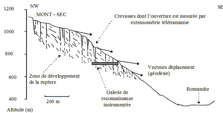
Figure 5. Schematic section of the Séchilienne slope movement. [Source: Pierre Antoine, André Giraud, Jean-Marc Vengeon, 1999. http://www.risknat.org/projets/cper/projets_1994-1999/04-Vengeon_&_al_2000-Sechilienne.pdf ]
