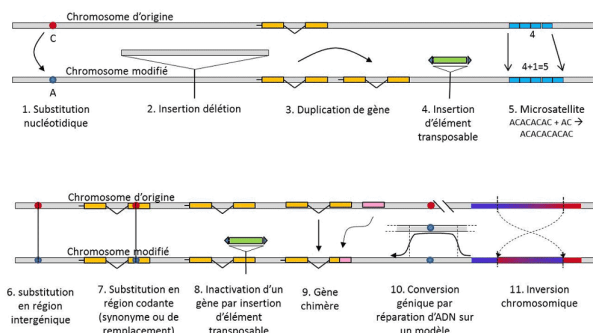
Figure 3. Different types of mutations. 1, nucleotide substitution, affecting a base (A, C, G, or T); 2, insertion or deletion of a DNA fragment; 3, duplication of a gene; 4, insertion of a transposable element; 5, elongation or shortening of a microsatellite locus; 6, substitution in an intergenic region (silent or not); 7, substitution in a coding region (synonymous or amino acid replacement); 8, inactivation of a gene by insertion of a transposable element; 9, creation of a chimeric gene by combination of two coding regions; 10, gene conversion by repair of damaged DNA, using another allele as a model; 11, chromosome inversion.
