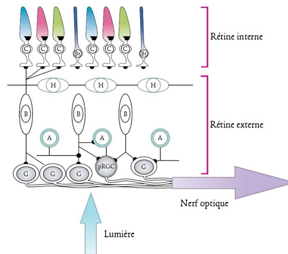
Figure 4. Transmission of photic information. In mammals, the photons that make up light are absorbed by visual photoreceptors, cones (C) and rods (Bt), and non-visual, photosensitive ganglion cells (pRGC). The perceived information is then transmitted, via the optic nerve, to the lateral geniculate body for the treatment of visual photoreception and to the suprachiasmatic nucleus (biological clock) for the treatment of non-visual photoreception. The horizontal (H), bipolar (B), ganglionic (G) and amacrine (A) cells located in the retina participate in the transfer of photic information from the photoreceptors to the optic nerve. [Source: Modified figure [4] from Arendt [3]].
